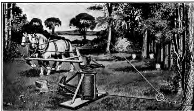
Fig. 29. Capstan Horse-Power Puller Made by Faultless Stump Puller Co., Cresco, Iowa
